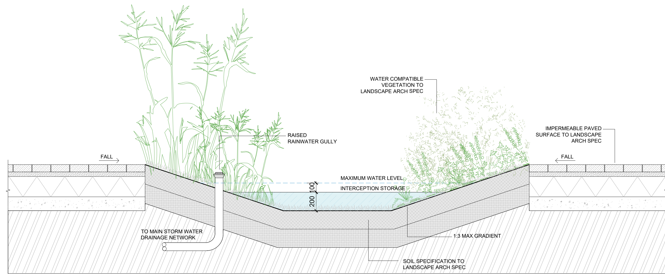
01 TYPICAL RAIN GARDEN DETAIL SCALE: 1:20 @A1
